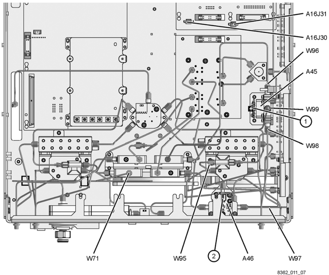
Figure 11 Cable Installation, Analyzers with Options UNL, 014, and 080
