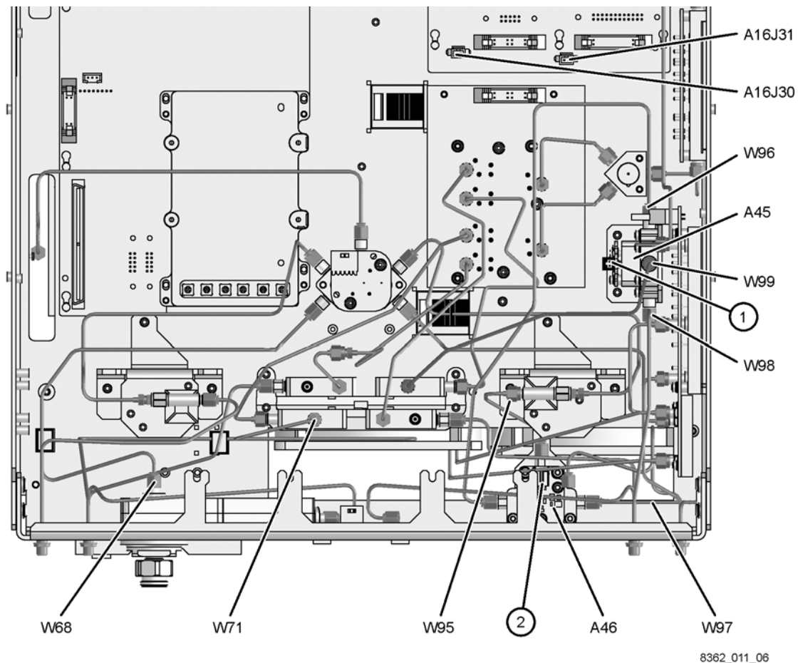
Figure 10 Cable Installation, Analyzers with Options 014 and 080
