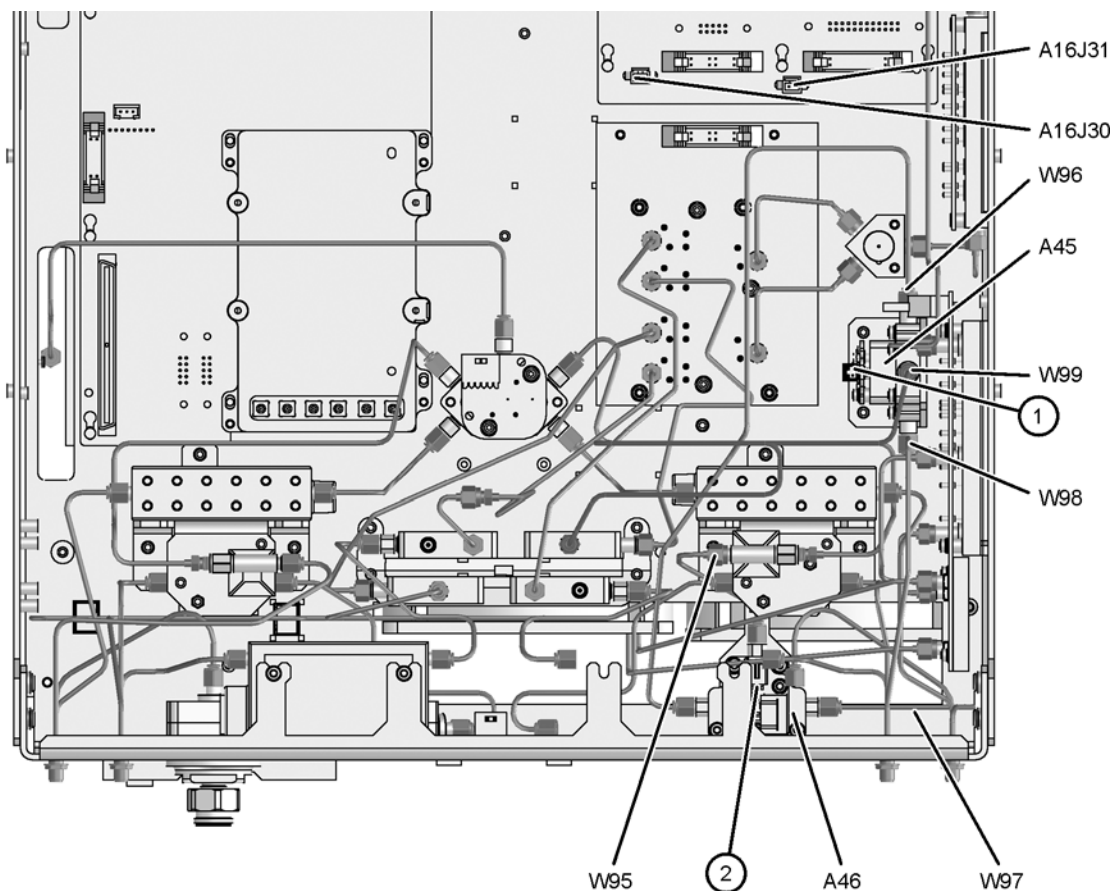
Figure 12 Cable Installation, Analyzers with Options UNL, 014, 016, and 080
