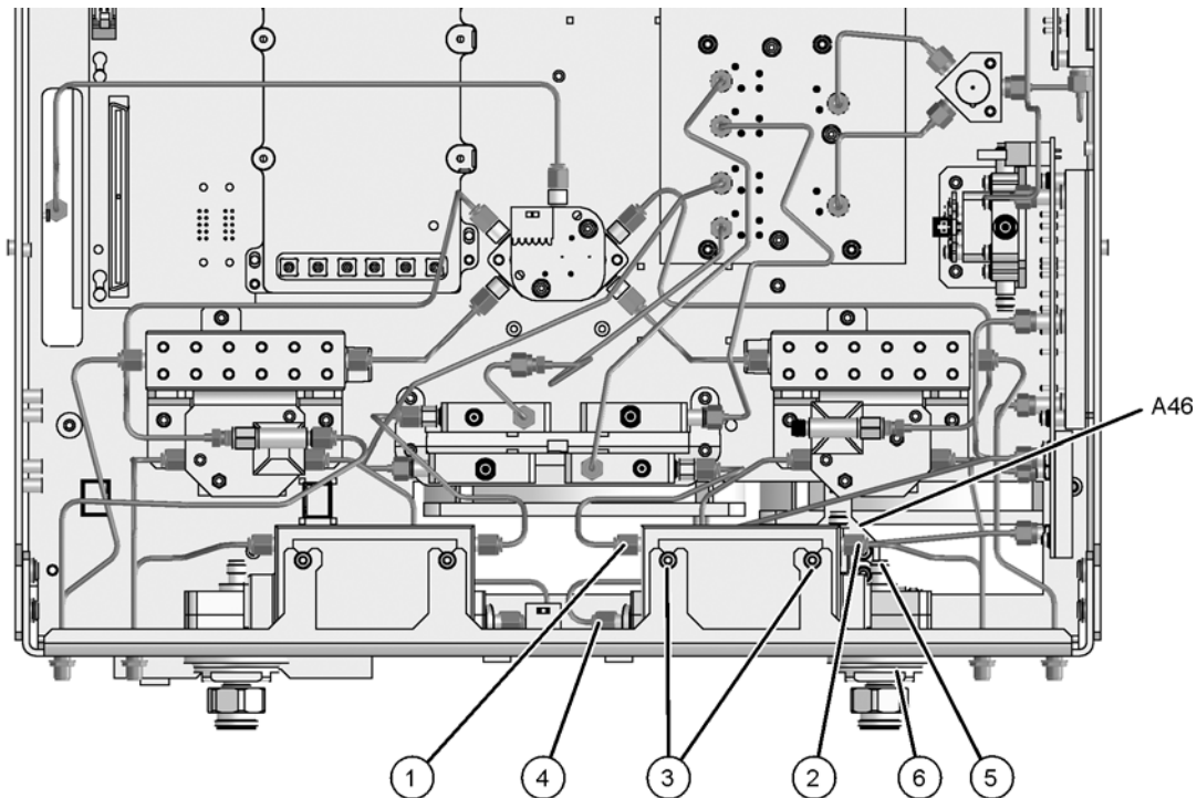
Figure 9 A46 Reference Switch Installation
