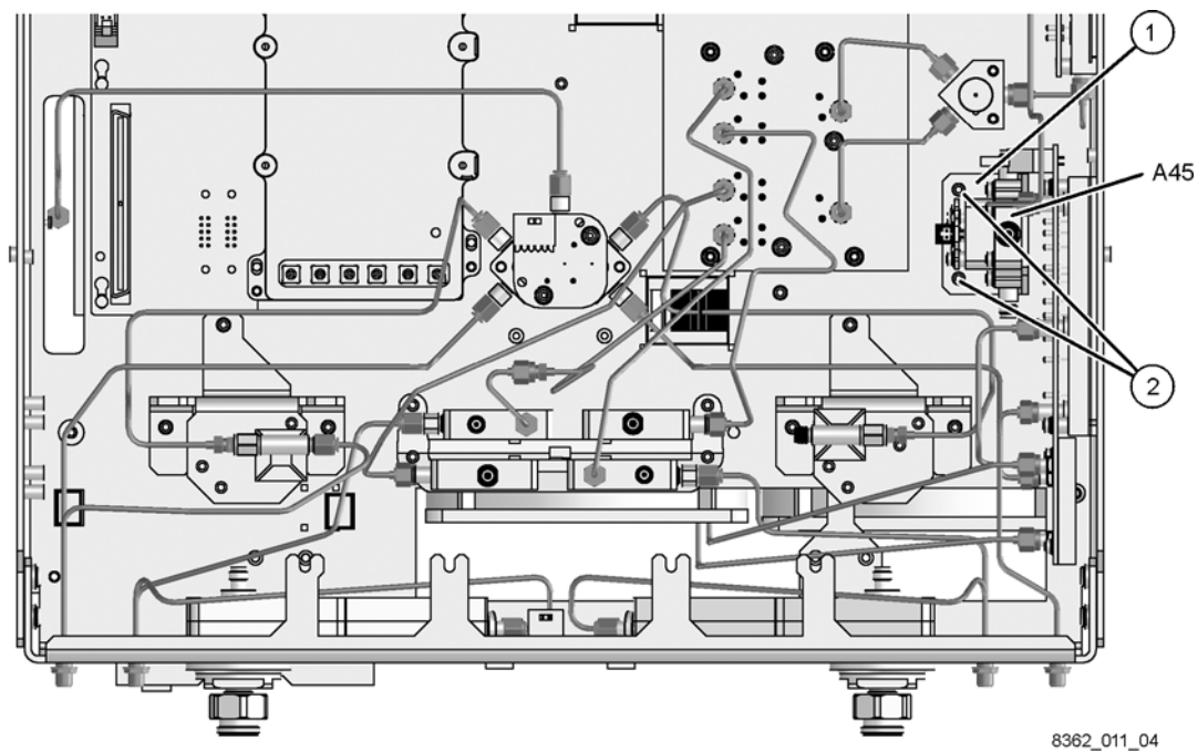
Figure 8 A45 Reference Switch Installation
