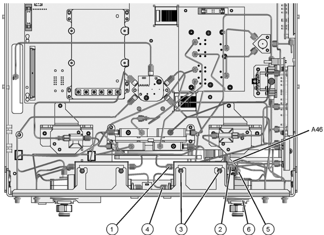
Figure 13 Test Port Coupler and Receiver Attenuator Reinstallation
